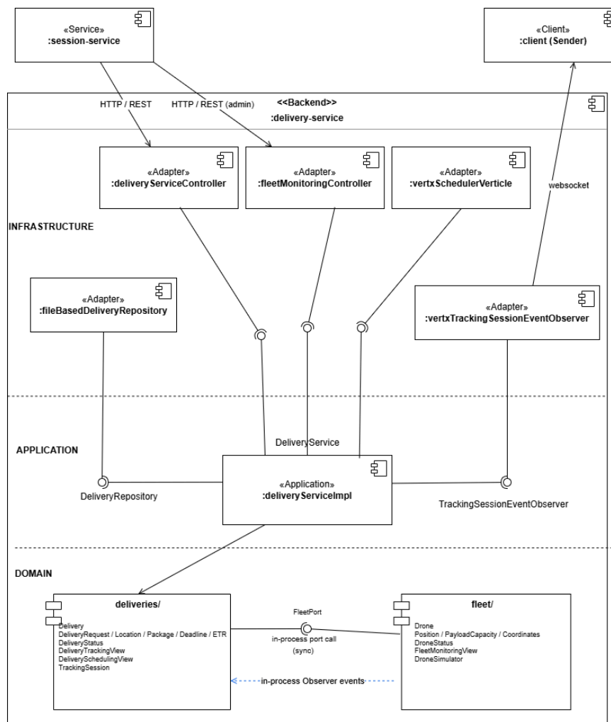
C&C diagram del delivery service (Deliveries + Fleet)
